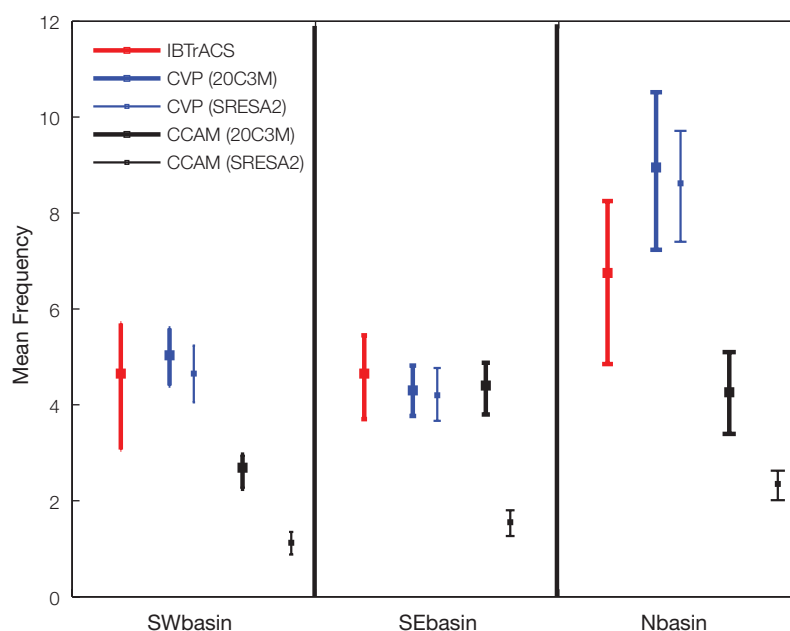
Figure 7.19: Average of all models of the late 21st century projected annual tropical cyclone frequency for the three sub-basins of the PCCSP region using the CCAM downscaling technique (thin black) and the Curvature Vorticity Parameter (CVP) method (thin blue). Also shown are the annual cyclone frequencies for the current climate for the CCAM downscaling technique (thick black) and the CVP method (thick blue). Red lines indicate observed mean tropical cyclone frequency. Bars denote 95% confidence interval. A change is considered likely if there is no overlap between current and future climate bars. Results are based on outputs from the CSIRO-Mk3.5, ECHAM5/MPI-OM, GFDL-CM2.0 and GFDL-CM2.1 global climate models (CVP) and CCAM simulations based on these global models.
