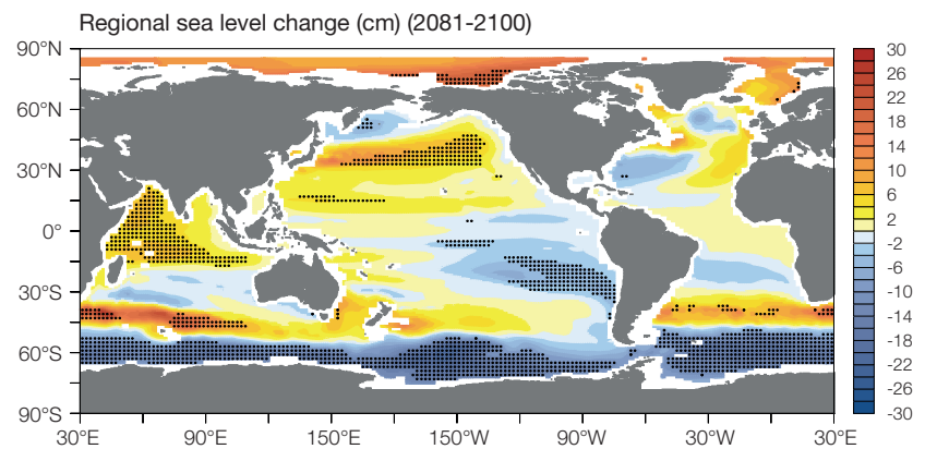
Figure 6.24: The global distribution of regional sea-level change (in cm) due to ocean density and circulation change during 2081–2100 relative to 1981–2000, derived from 13 available CMIP3 models subjected to the A1B (medium) scenario. The global mean is removed, thus positive (negative) values indicate higher (lower) local sea-level change than global average. Stippling denotes that regions where climate models tend to agree, defined as the regions where the magnitude of multi-model mean exceeds the inter-model standard deviation.
