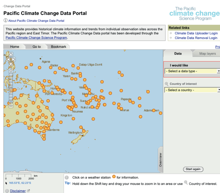
Figure 2.1: Locations of surface observed data stations in the Pacific Climate Change Data Portal http://www.bom.gov.au/climate/pccsp/ .
