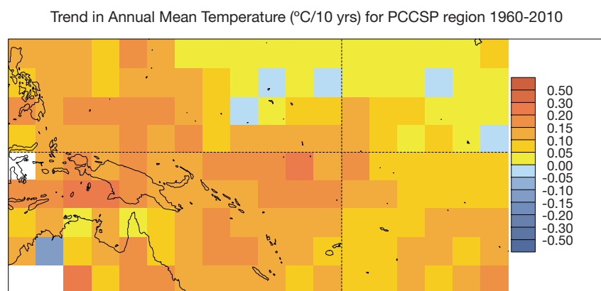
Figure 3.2: Trend in annual mean temperature (°C per decade) over 1960–2010, as determined by the HadCRUT3v global gridded temperature dataset (Brohan et al., 2006).
