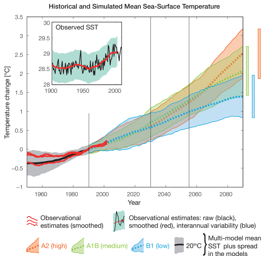
Figure 10.7: Historical climate (from 1950 onwards) and simulated historical and future climate for annual mean sea-surface temperature (SST) in the region surrounding Palau, for the CMIP3 models. Shading represents approximately 95% of the range of model projections (twice the inter-model standard deviation), while the solid lines represent the smoothed (20-year running average) multi-model mean temperature. Projections are calculated relative to the 1980–1999 period (which is why there is a decline in the inter-model standard deviation around 1990). Observational estimates in the main figure (red lines) are derived from the HadSST2, ERSST and Kaplan Extended SST V2 datasets (Volume 1, Section 2.2.2). Annual average (black) and 20-year running average (red) HadSST2 data is also shown inset.
