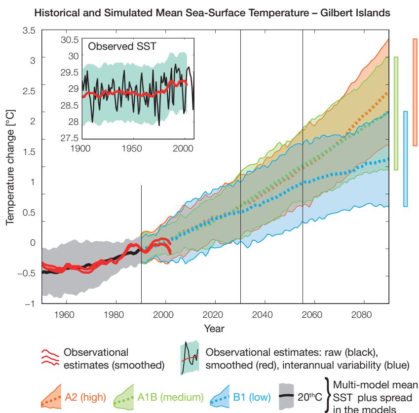
Figure 6.7: Historical climate (from 1950 onwards) and simulated historical and future climate for annual mean sea-surface temperatures (SST) in the region surrounding the Gilbert Islands for the CMIP3 models. Shading represents approximately 95% of the range of model projections (twice the inter-model standard deviation), while the solid lines represent the smoothed (20-year running average) multi-model mean temperature. Projections are calculated relative to the 1980–1999 period (which is why there is a decline in the inter-model standard deviation around 1990). Observational estimates in the main figure (red lines) are derived from the HadSST2, ERSST and Kaplan Extended SST V2 datasets (Volume 1, Section 2.2.2). Annual average (black) and 20-year running average (red) HadSST2 data is also shown inset. Projections for the Phoenix and Line Islands closely resemble those of the Gilbert Islands and are therefore not shown.
