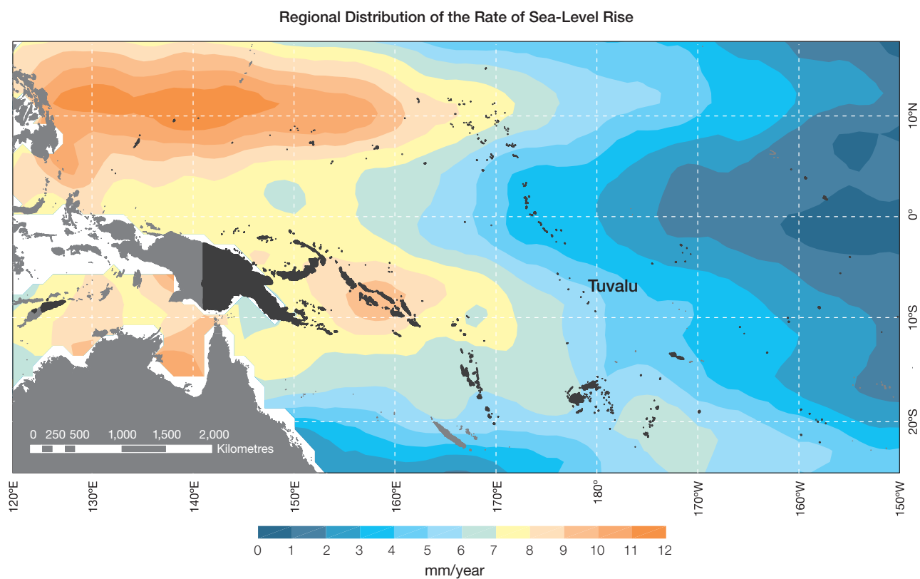
Figure 15.6: The regional distribution of the rate of sea-level rise measured by satellite altimeters from January 1993 to December 2010, with the location of Tuvalu indicated. Further detail about regional distribution of sea-level rise is provided in Volume 1, Section 3.6.3.2.
