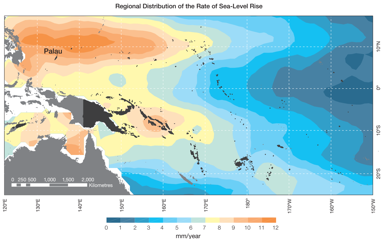
Figure 10.5: The regional distribution of the rate of sea-level rise measured by satellite altimeters from January 1993 to December 2010, with the location of Palau indicated. Further detail about the regional distribution of sea-level rise is provided in Volume 1, Section 3.6.3.2.
