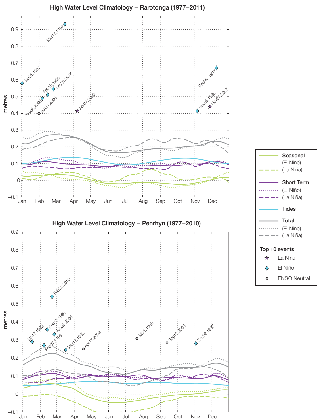
Figure 2.7: The annual cycle of high waters relative to Mean Higher High Water (MHHW) due to tides, short-term fluctuations (most likely associated with storms) and seasonal variations for Rarotonga (top) and Penrhyn (bottom). The tides and short-term fluctuations are respectively the 95% exceedence levels of the astronomical high tides relative to MHHW and the short-term sea level anomaly fluctuations. Components computed only for El Niño and La Niña years are shown by dotted and dashed lines, and grey lines are the sum of the tide, short-term and seasonal components. The 10 highest sea level events in the record relative to MHHW are shown, and coded to indicate the phase of ENSO at the time of the extreme event.
