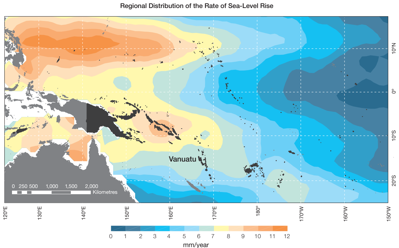
Figure 16.6: The regional distribution of the rate of sea-level rise measured by satellite altimeters from January 1993 to December 2010, with the location of Vanuatu indicated. Further detail about the regional distribution of sea-level rise is provided in Volume 1, Section 3.6.3.2.
