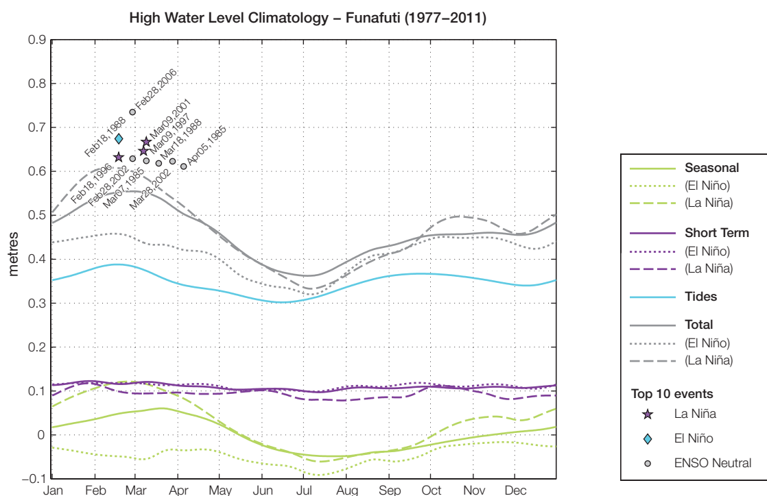
Figure 15.7: The annual cycle of high waters relative to Mean Higher High Water (MHHW) due to tides, short-term fluctuations (most likely associated with storms) and seasonal variations for Tuvalu. The tides and short-term fluctuations are respectively the 95% exceedence of the astronomical high tides relative to MHHW and short-term sea level fluctuations. Components computed only for El Niño and La Niña months are shown by dotted and dashed lines, and grey lines are the sum of the tide, short-term and seasonal components. The 10 highest sea-level events in the record relative to MHHW are shown, and coded to indicate the phase of ENSO at the time of the extreme event.
