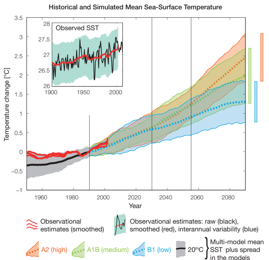
Figure 16.8: Historical climate (from 1950 onwards) and simulated historical and future climate for annual mean sea-surface temperature (SST) in the region surrounding Vanuatu, for the CMIP3 models. Shading represents approximately 95% of the range of model projections (twice the inter-model standard deviation), while the solid lines represent the smoothed (20-year running average) multi-model mean temperature. Projections are calculated relative to the 1980–1999 period (which is why there is a decline in the inter-model standard deviation around 1990). Observational estimates in the main figure (red lines) are derived from the HadSST2, ERSST and Kaplan Extended SST V2 datasets (Volume 1, Section 2.2.2). Annual average (black) and 20-year running average (red) HadSST2 data is also shown inset.
