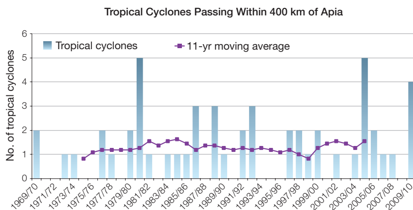
Figure 12.5: Tropical cyclones passing within 400 km of Apia per season. The 11-year moving average is in purple.
